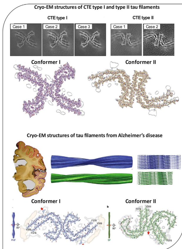
Figure 3. Near-atomic resolution applications of cryo-EM technology
